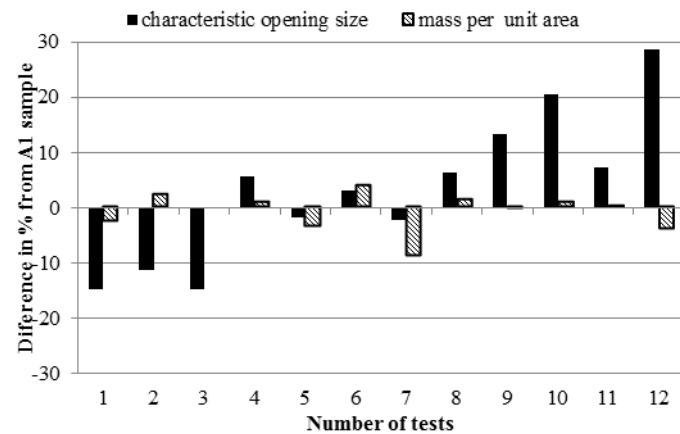
Figure 5. EN ISO 12956 Characteristic opening size
