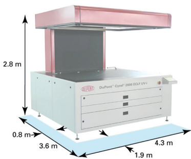
Floor Plan
